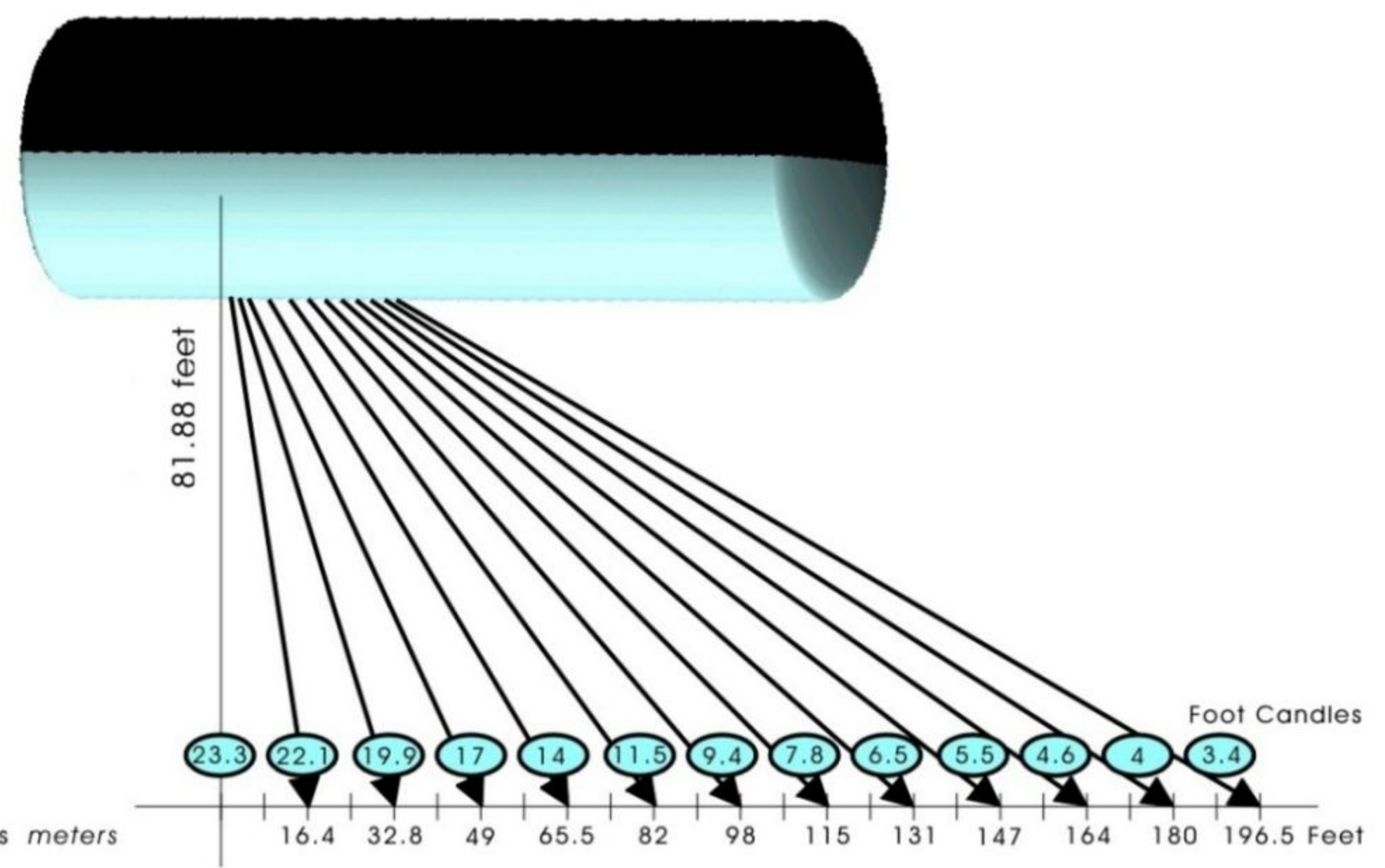
Tube 2400 HH Lighting Chart
