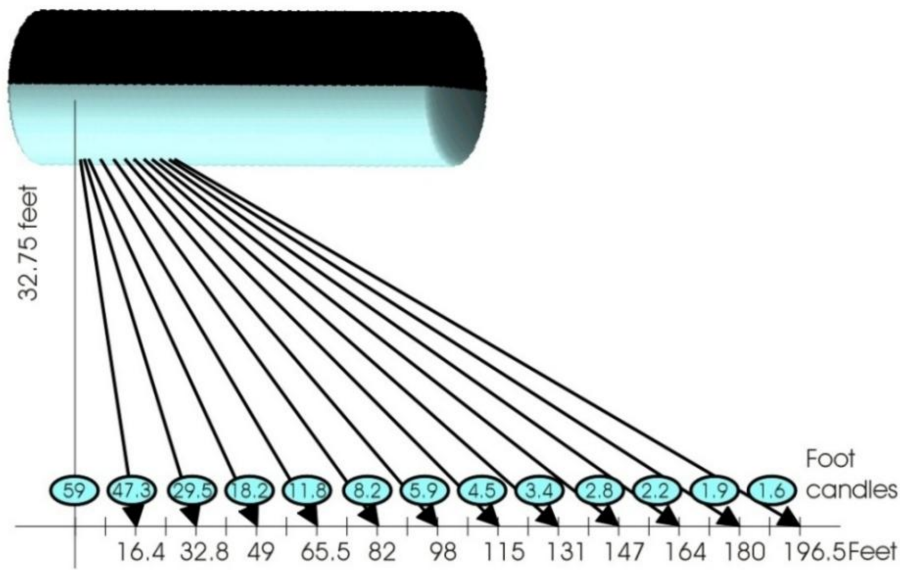
Tube 1280 HH Lighting Chart
