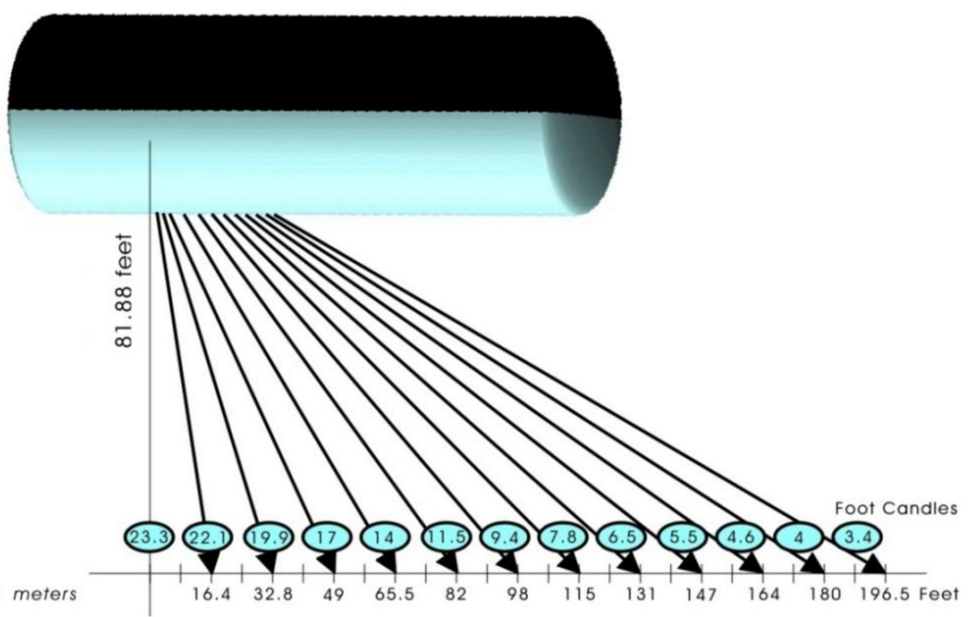
Tube 2400 HH Lighting Chart
