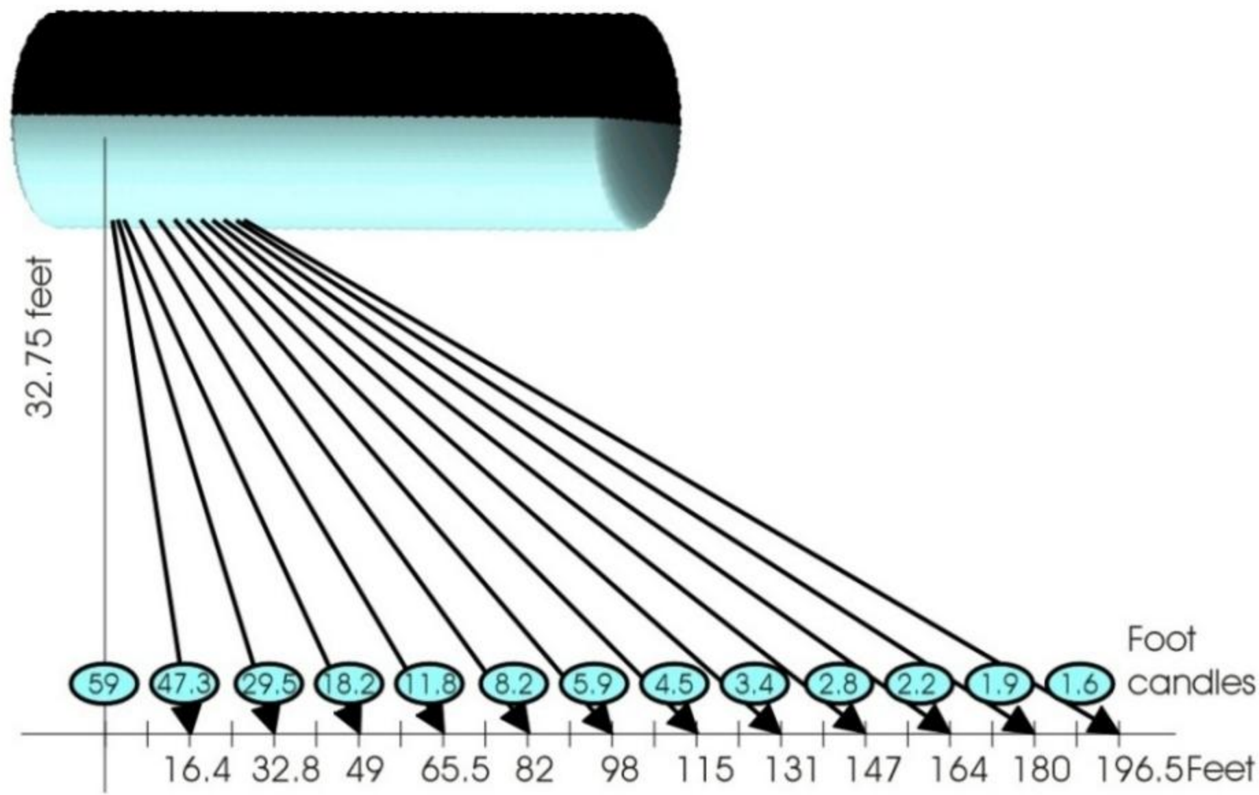
Tube 1280 HH Lighting Chart
