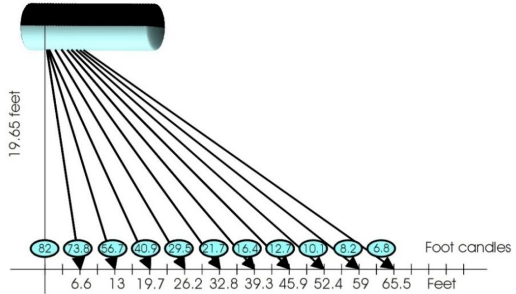
Tube 440 HH Lighting Chart
