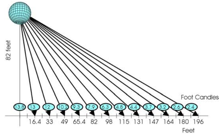
Solarc 700 HMI Lighting Chart
