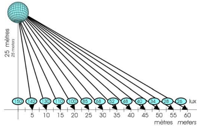
Flux lumineux Solarc 700 HMI
